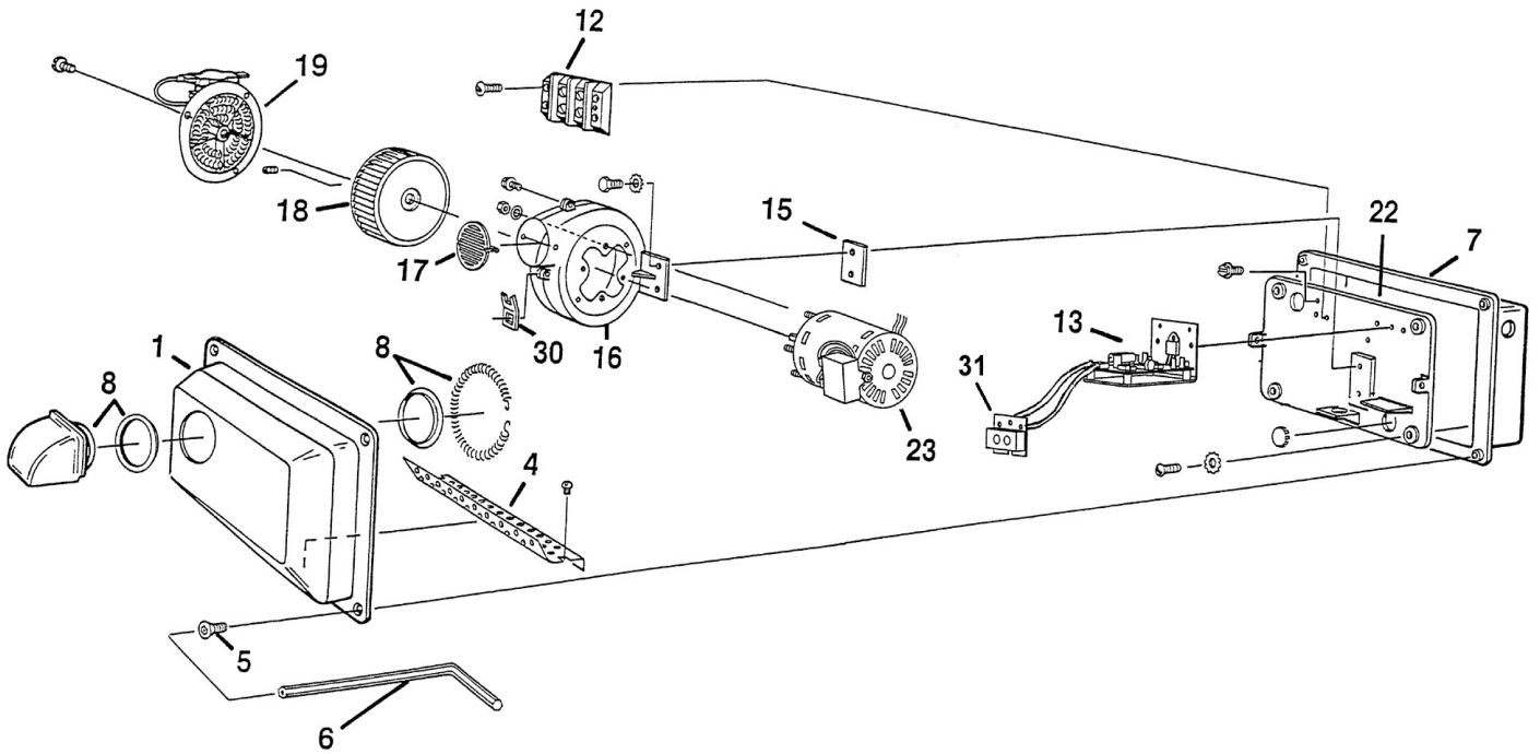
Recessed Mounted with Triac Control
